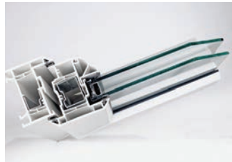
Window Cross Section
